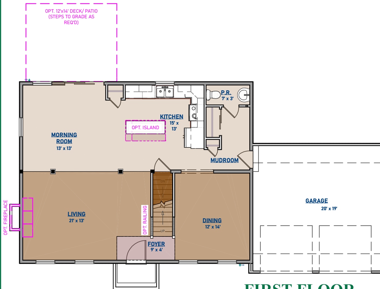
FIRST FLOOR
