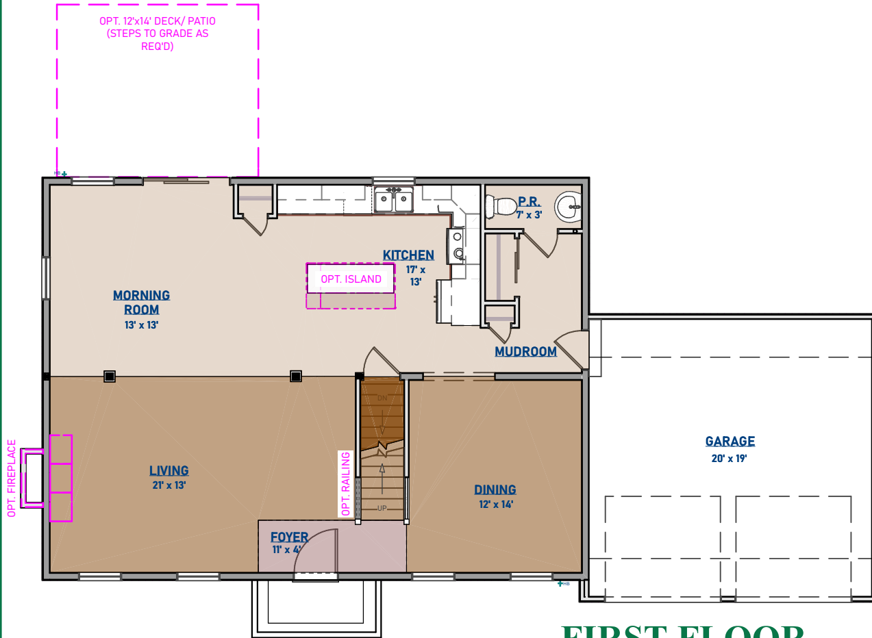
FIRST FLOOR
